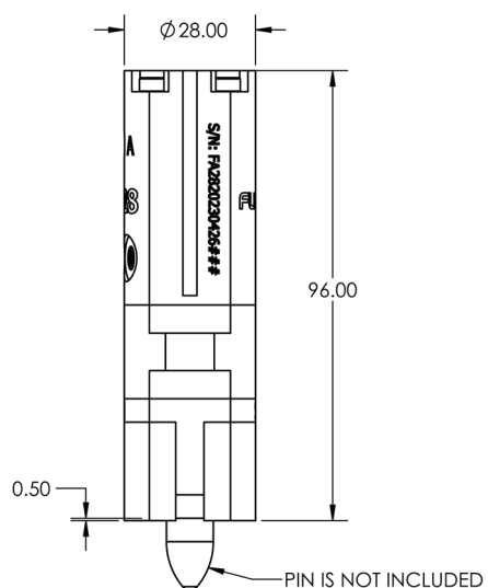
FA28 Standard Pin Pole
