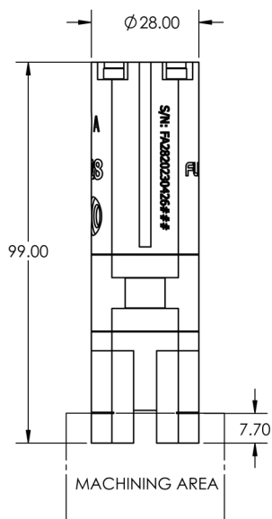
FA28 Standard Blank Pole
